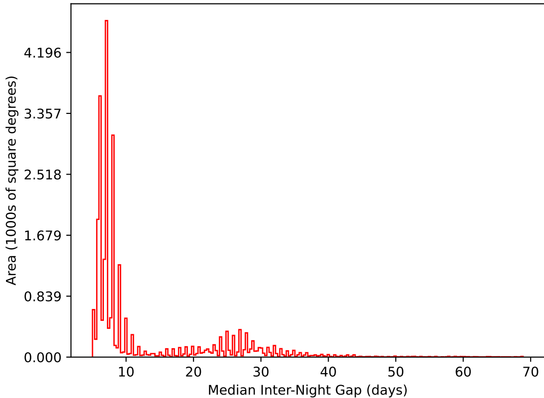
too_ignore_5_1v3.4_10yrs All sky i band: Median Inter-Night Gap
