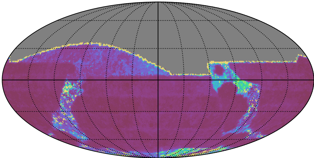
too_ignore_5_1v3.4_10yrs All sky g band: Median Inter-Night Gap
