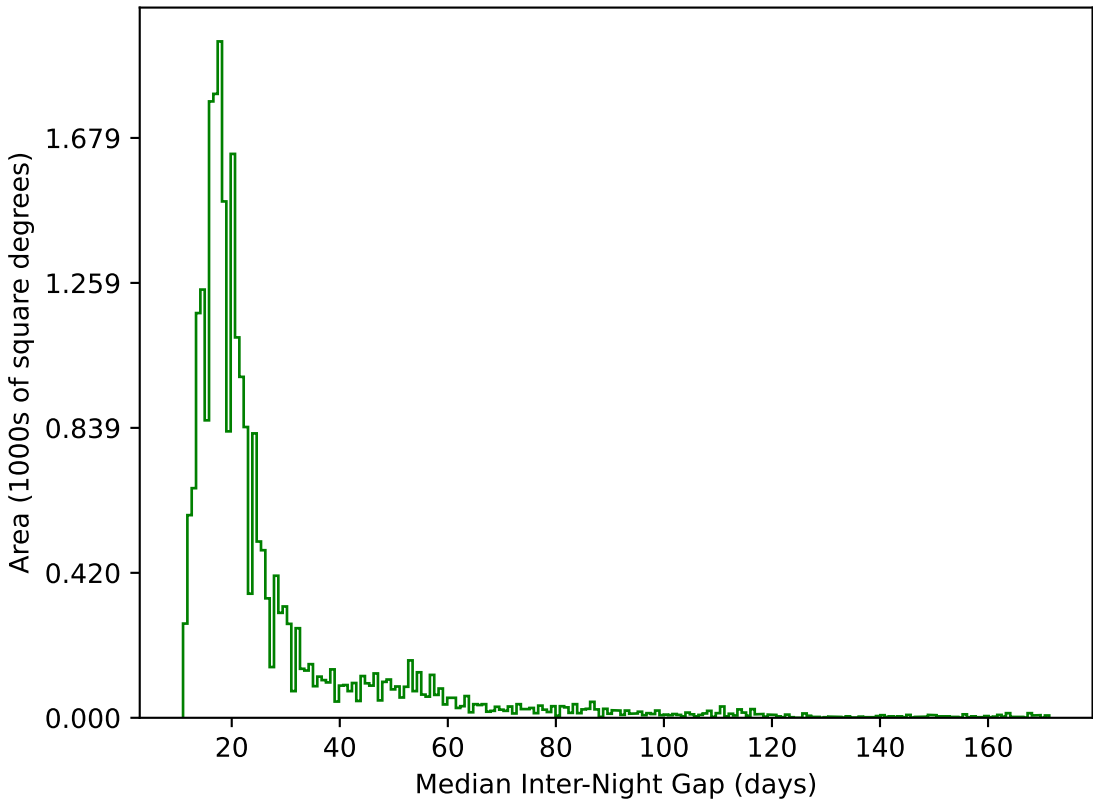
too_ignore_5_1v3.4_10yrs All sky g band: Median Inter-Night Gap
