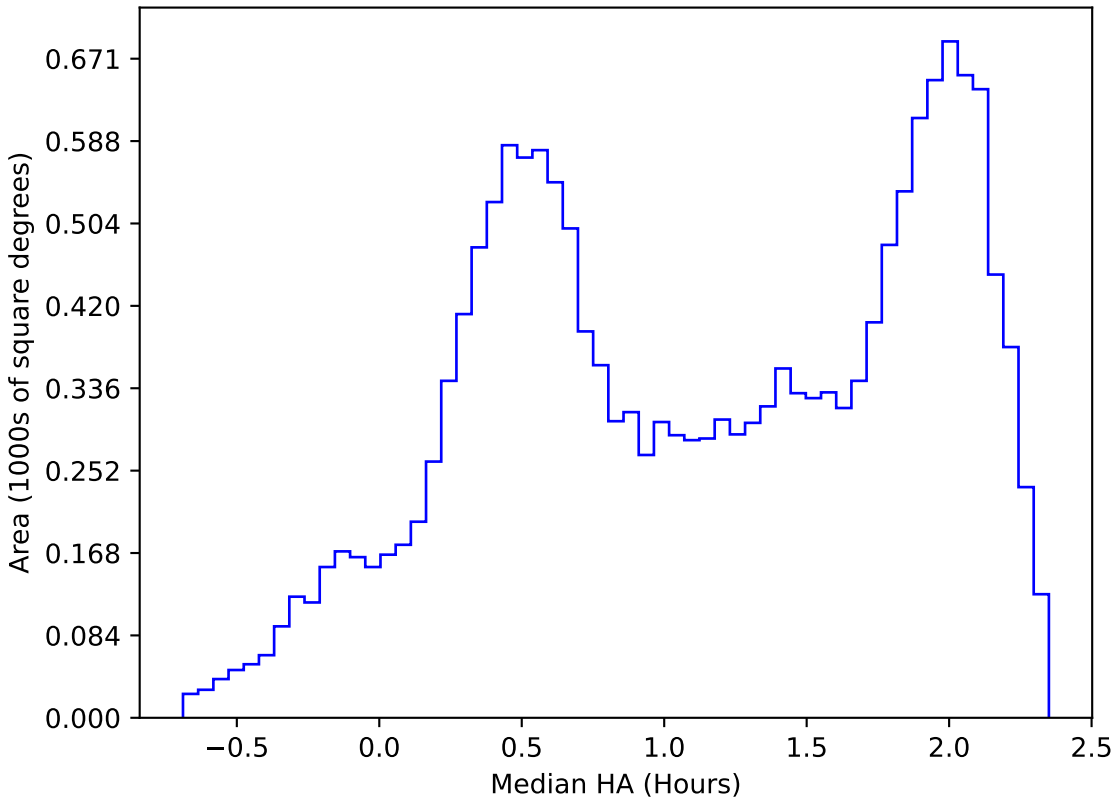
too_ignore_5_1v3.4_10yrs WFD z band: Median HA
