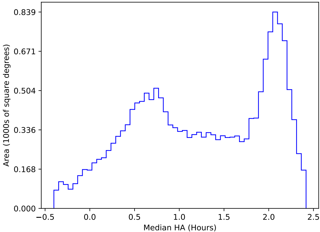
too_ignore_5_1v3.4_10yrs WFD y band: Median HA
