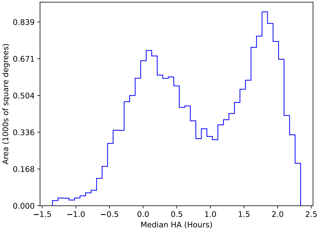
too_ignore_5_1v3.4_10yrs WFD u band: Median HA
