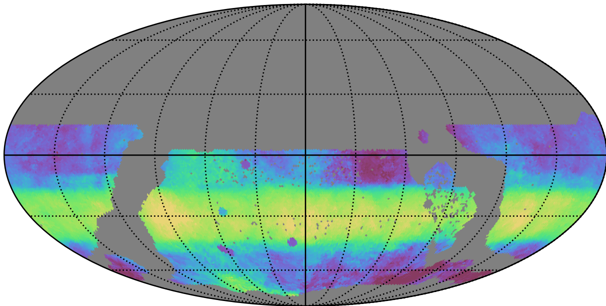
too_ignore_5_1v3.4_10yrs WFD i band: Median HA
