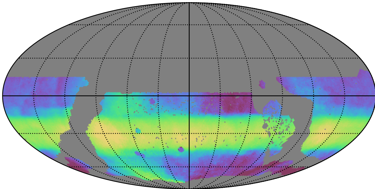
too_ignore_5_1v3.4_10yrs WFD all bands: Median HA
