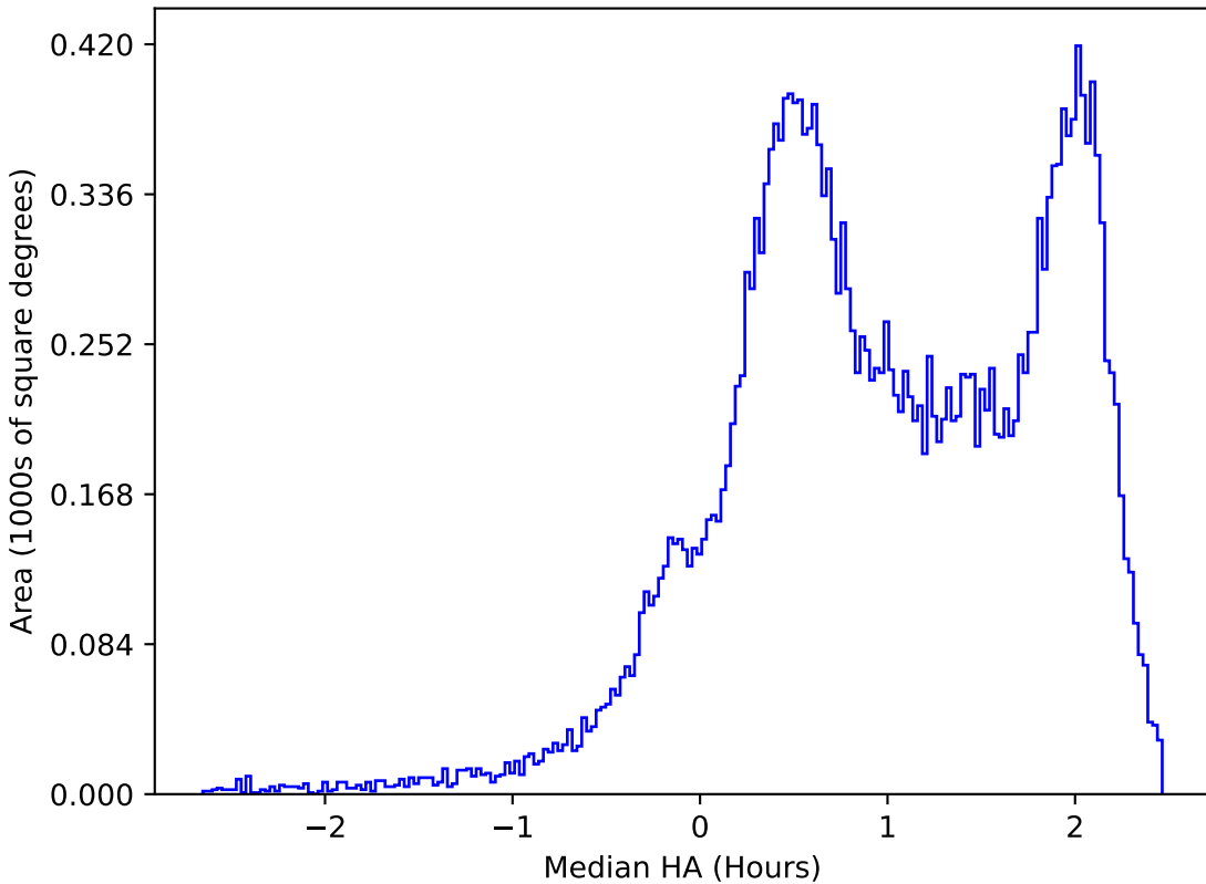
too_ignore_5_1v3.4_10yrs All sky z band: Median HA
