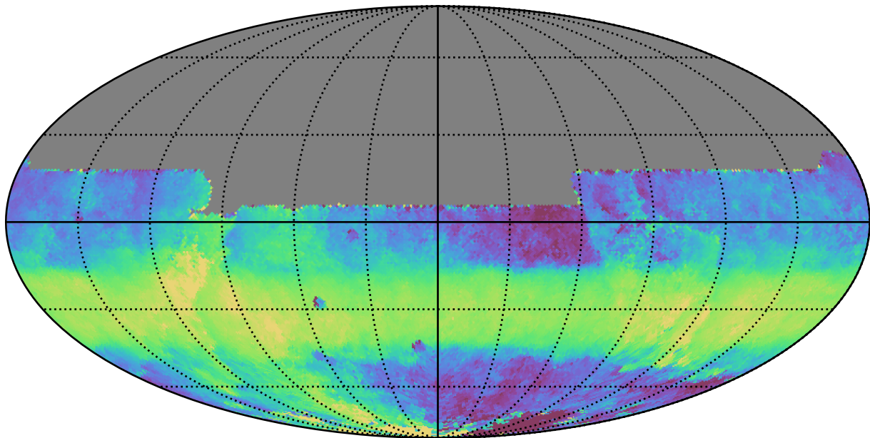
too_ignore_5_1v3.4_10yrs All sky y band: Median HA
