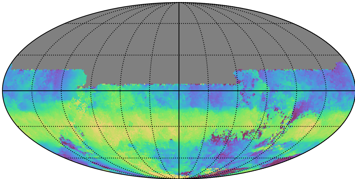
too_ignore_5_1v3.4_10yrs All sky u band: Median HA
