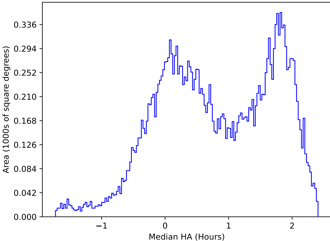
too_ignore_5_1v3.4_10yrs All sky u band: Median HA
