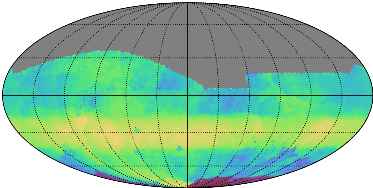
too_ignore_5_1v3.4_10yrs All sky r band: Median HA
