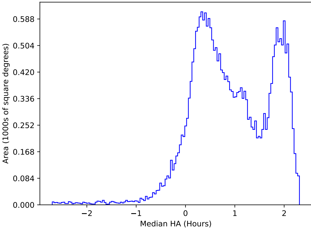
too_ignore_5_1v3.4_10yrs All sky i band: Median HA
