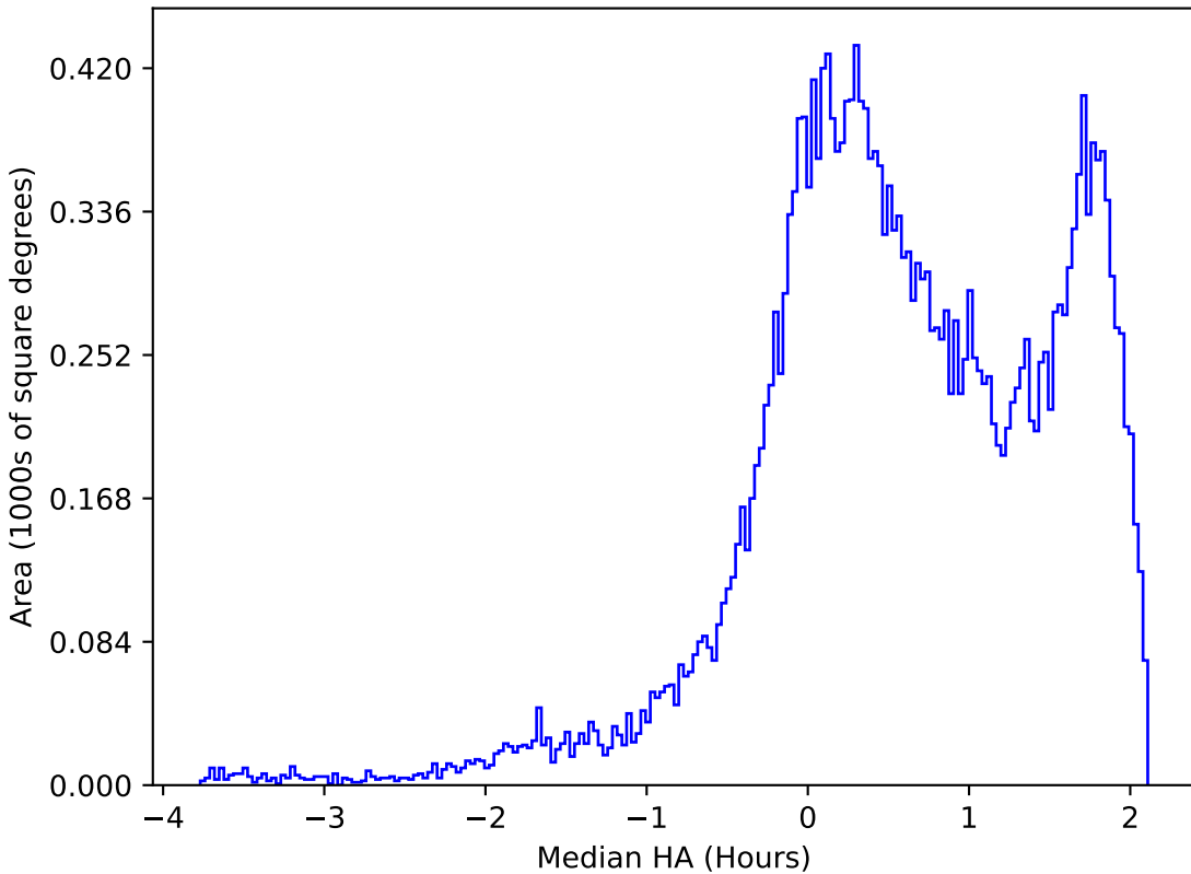
too_ignore_5_1v3.4_10yrs All sky g band: Median HA
