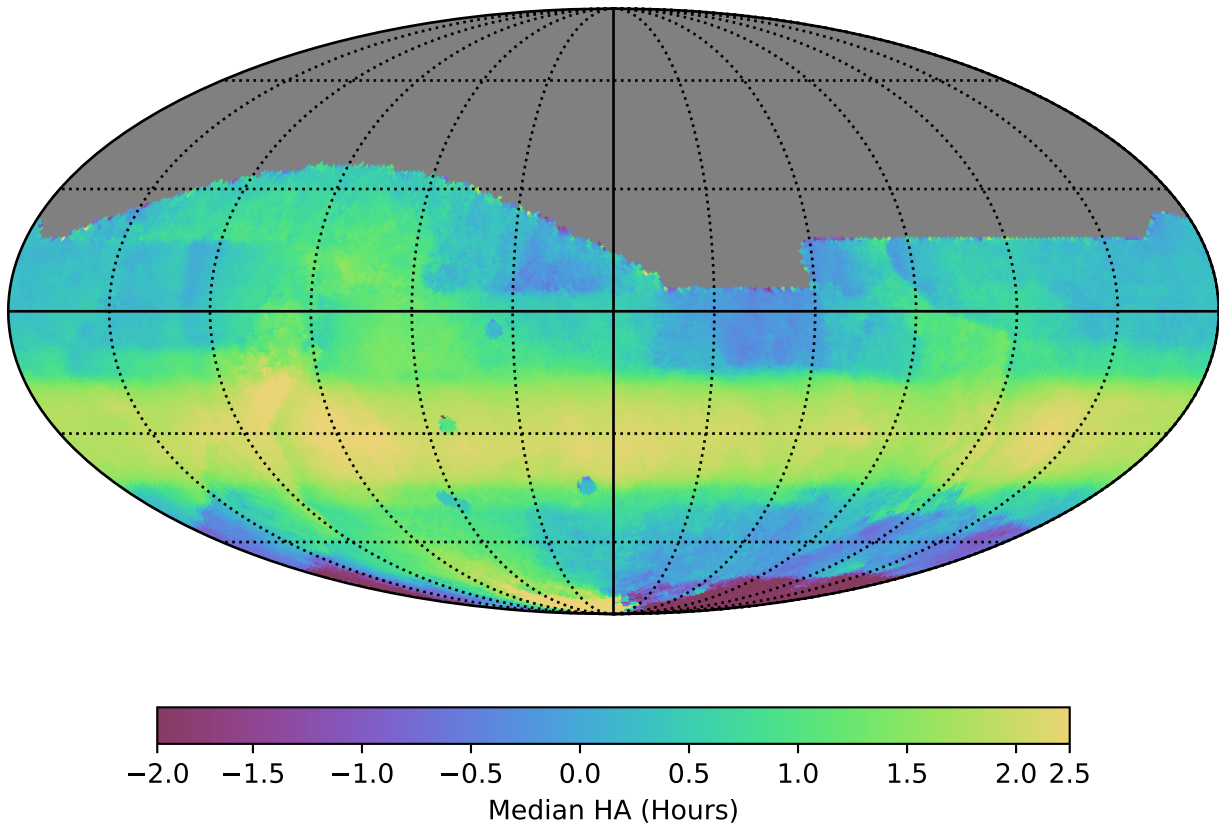
too_ignore_5_1v3.4_10yrs All sky all bands: Median HA
