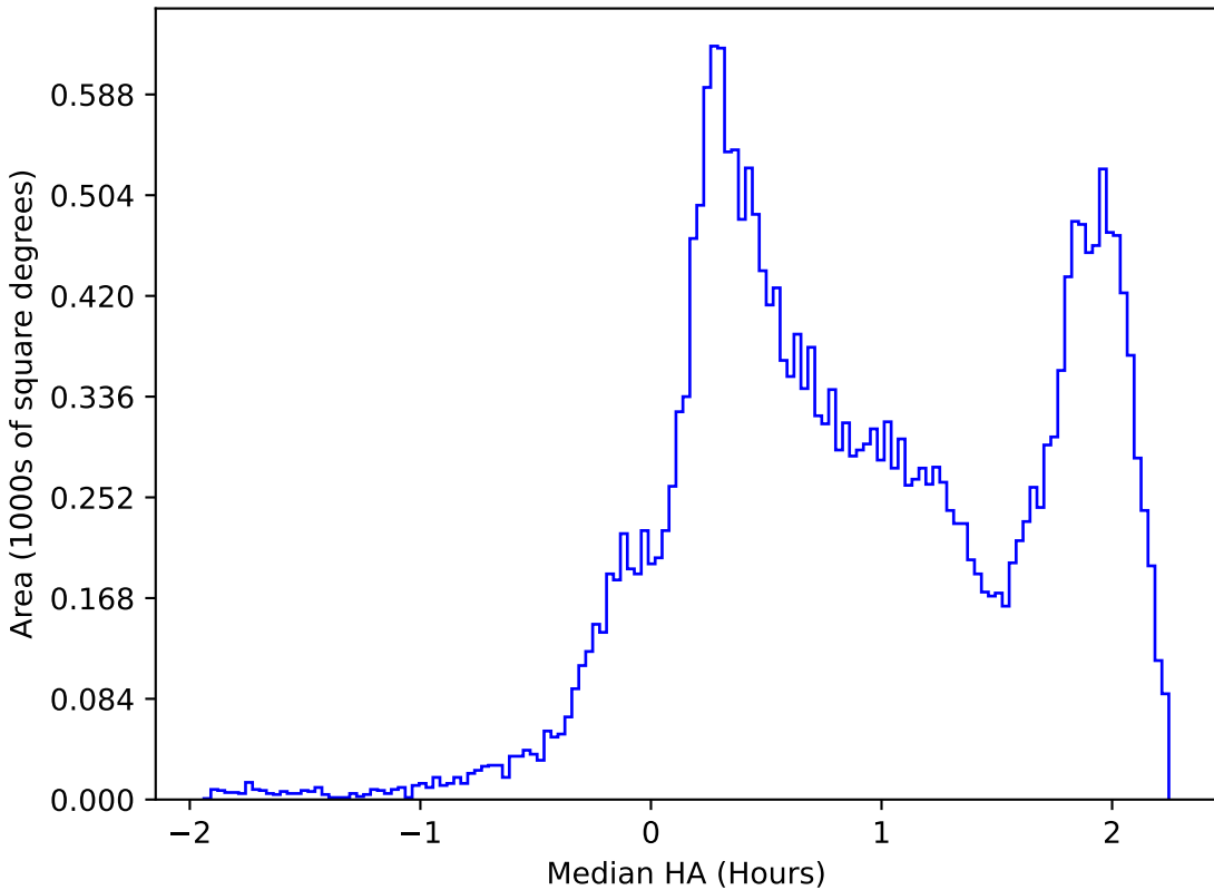
too_ignore_5_1v3.4_10yrs All sky all bands: Median HA
