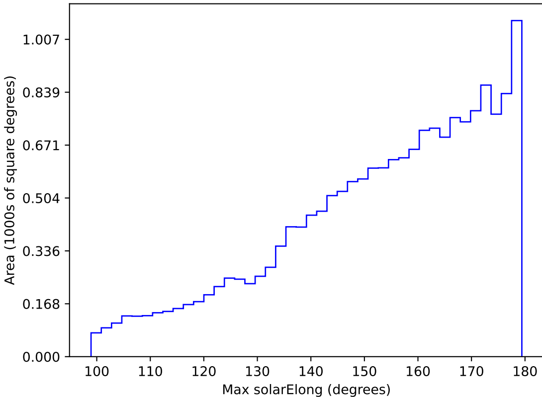
too_ignore_5_1v3.4_10yrs WFD z band: Max solarElong
