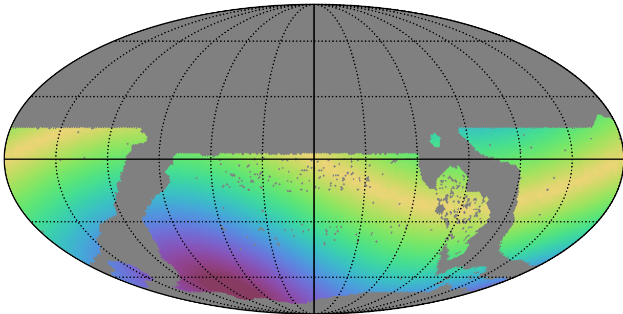
too_ignore_5_1v3.4_10yrs WFD r band: Max solarElong
