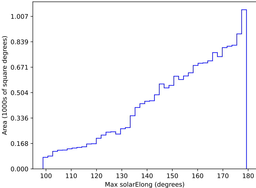
too_ignore_5_1v3.4_10yrs WFD r band: Max solarElong
