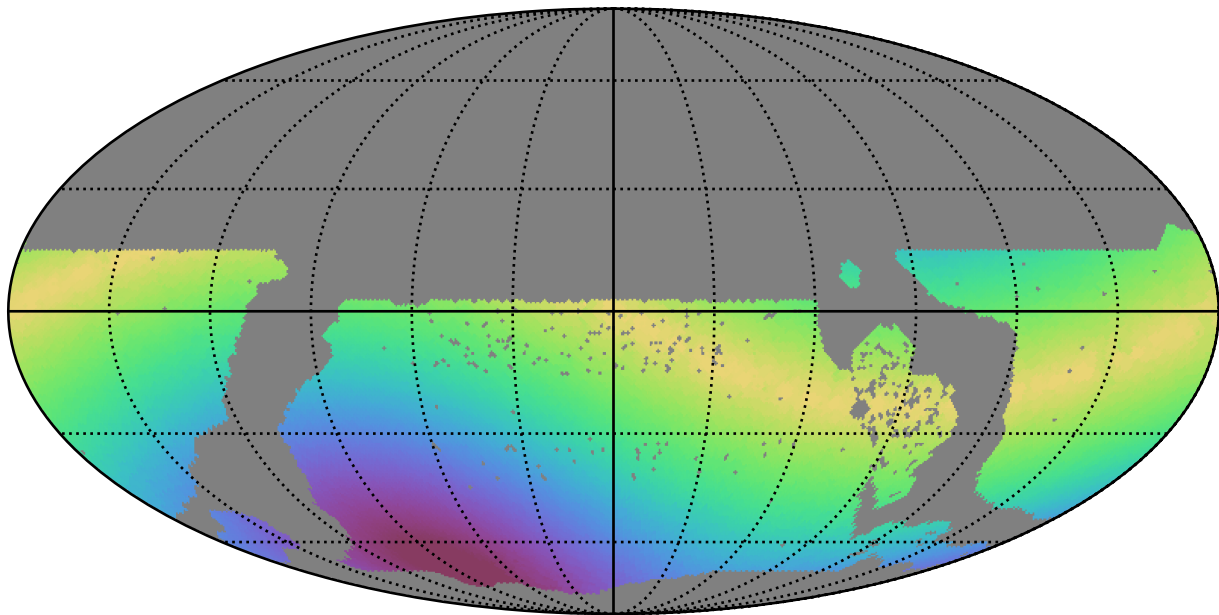
too_ignore_5_1v3.4_10yrs WFD g band: Max solarElong
