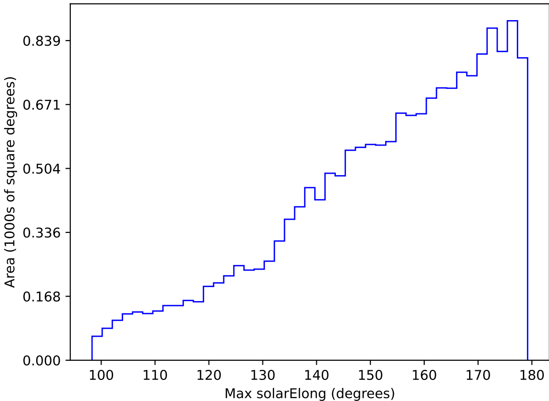
too_ignore_5_1v3.4_10yrs WFD g band: Max solarElong
