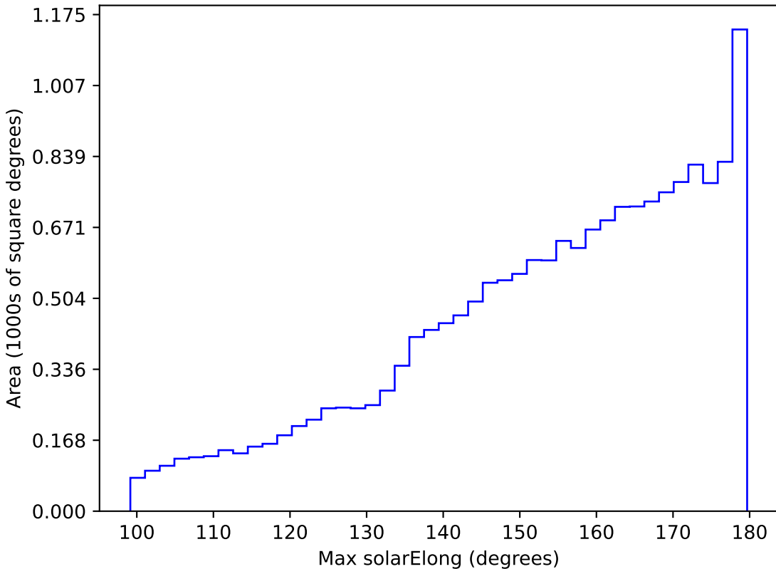
too_ignore_5_1v3.4_10yrs WFD all bands: Max solarElong
