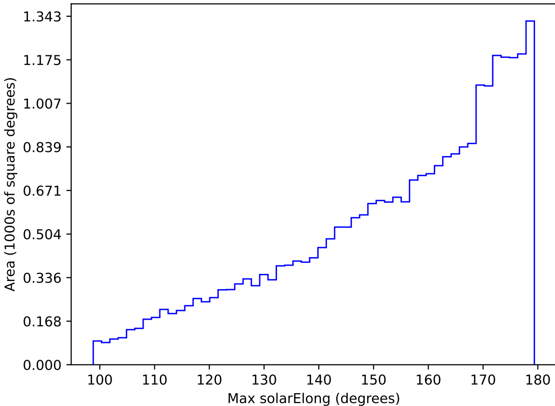
too_ignore_5_1v3.4_10yrs All sky z band: Max solarElong
