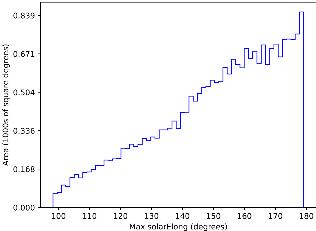
too_ignore_5_1v3.4_10yrs All sky y band: Max solarElong
