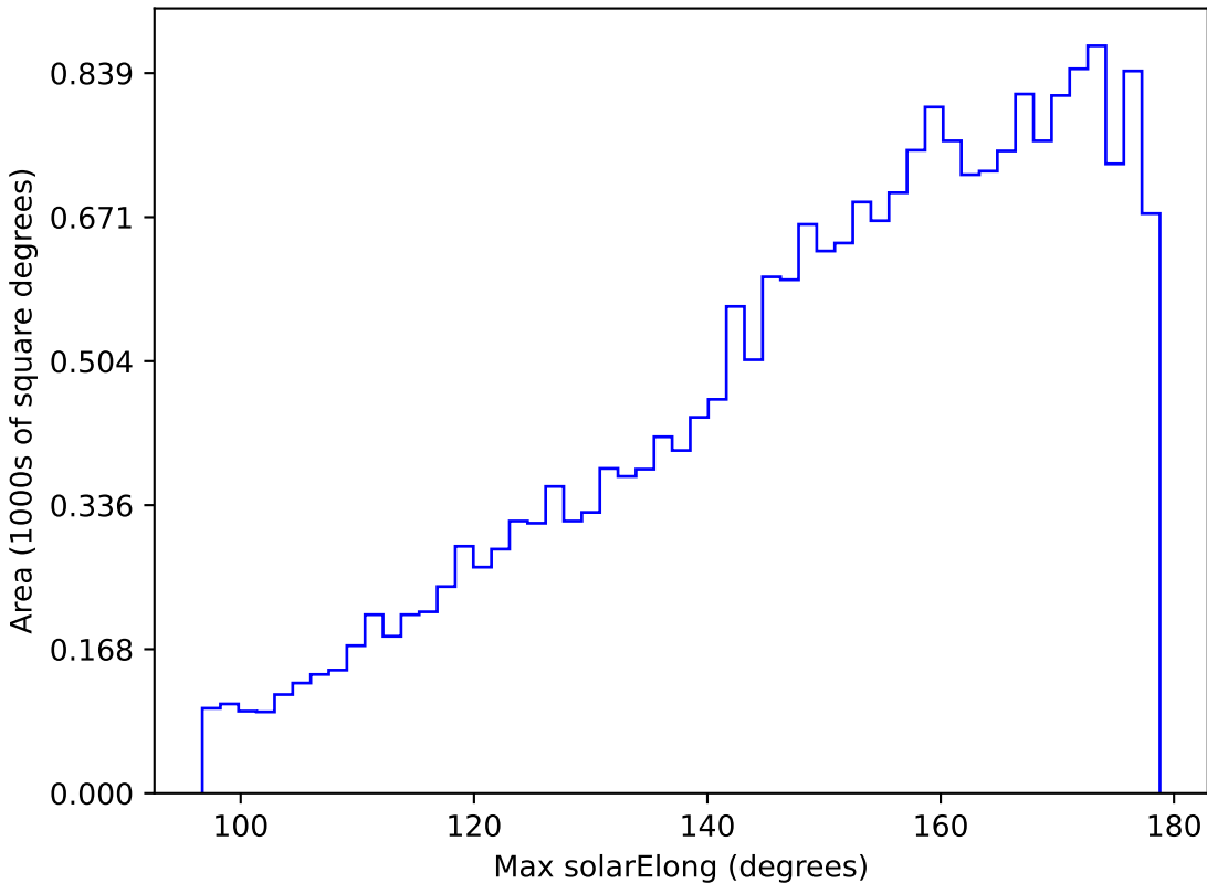
too_ignore_5_1v3.4_10yrs All sky u band: Max solarElong
