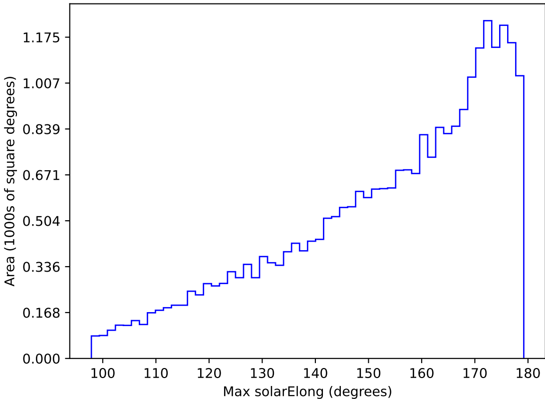
too_ignore_5_1v3.4_10yrs All sky g band: Max solarElong
