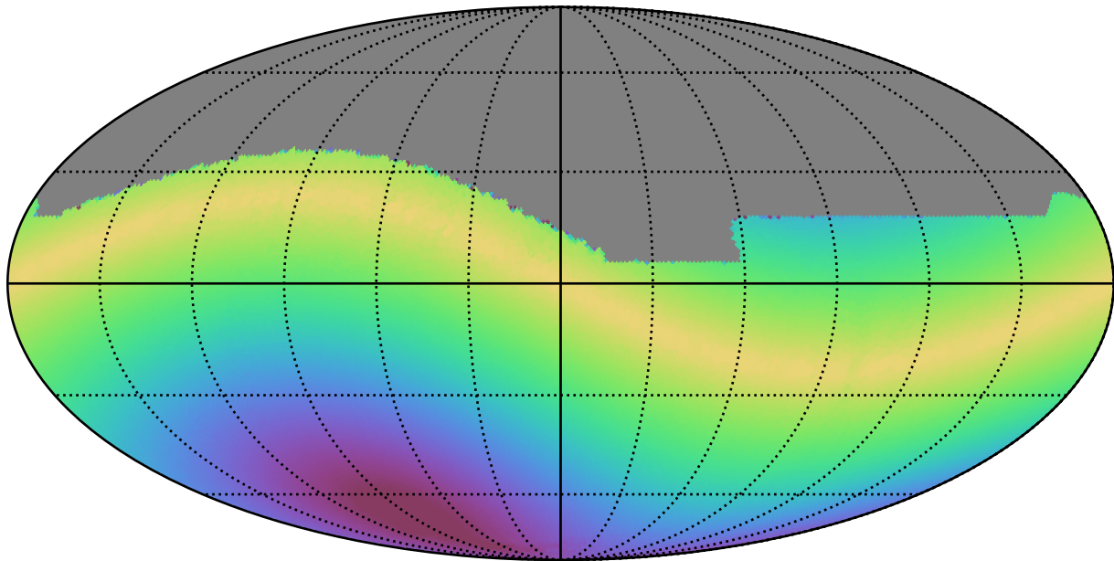
too_ignore_5_1v3.4_10yrs All sky all bands: Max solarElong
