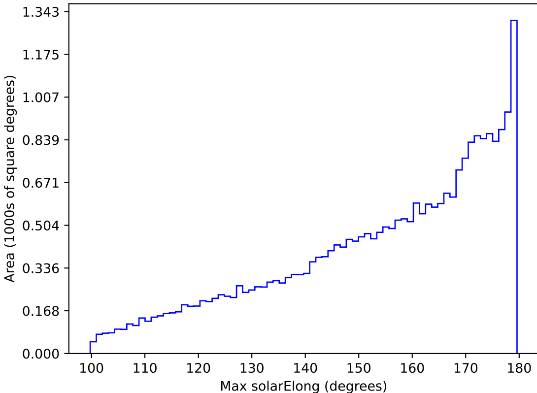
too_ignore_5_1v3.4_10yrs All sky all bands: Max solarElong
