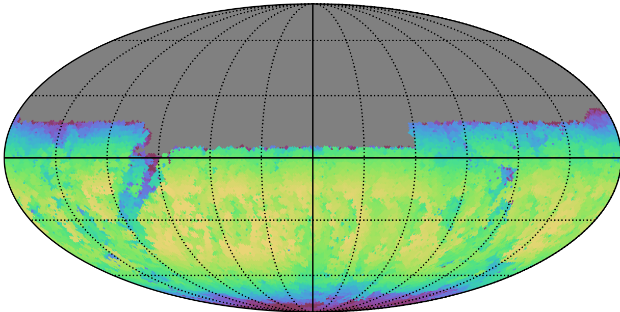
too_ignore_5_1v3.4_10yrs Yr 1 y band: Max skyBrightness
