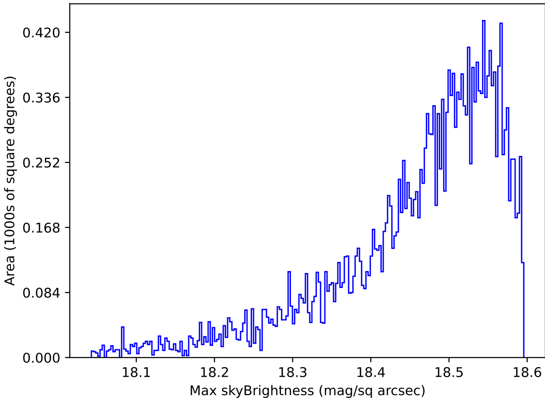
too_ignore_5_1v3.4_10yrs Yr 1 y band: Max skyBrightness
