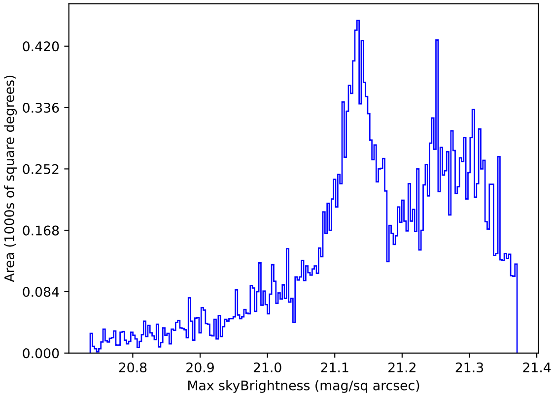
too_ignore_5_1v3.4_10yrs Yr 1 r band: Max skyBrightness
