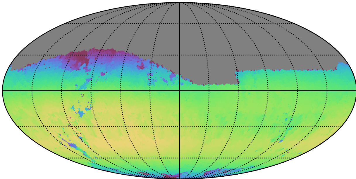
too_ignore_5_1v3.4_10yrs Yr 1 i band: Max skyBrightness
