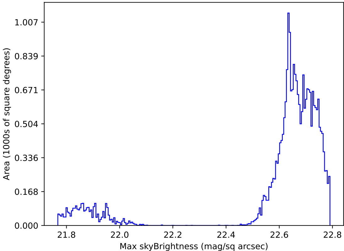
too_ignore_5_1v3.4_10yrs Yr 1 all bands: Max skyBrightness
