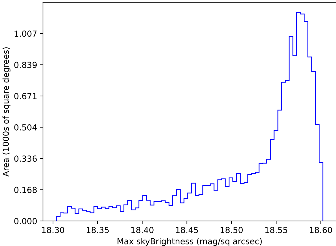
too_ignore_5_1v3.4_10yrs WFD y band: Max skyBrightness
