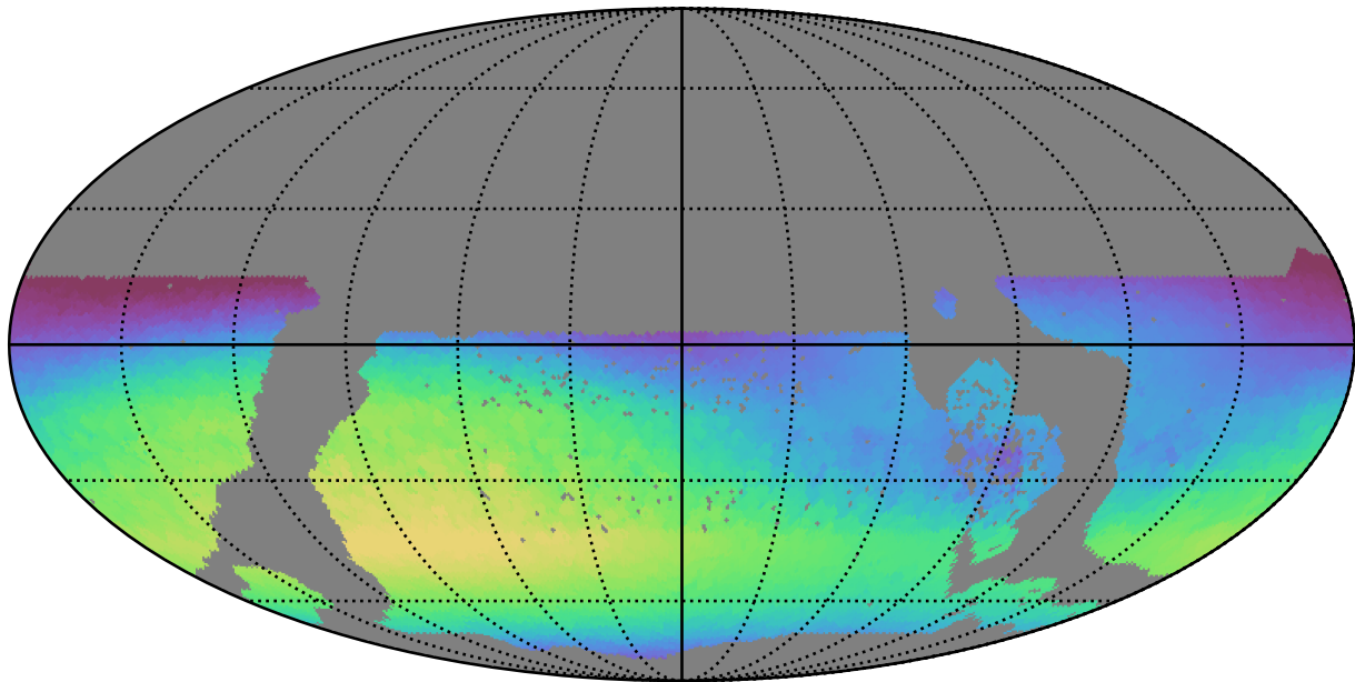
too_ignore_5_1v3.4_10yrs WFD u band: Max skyBrightness
