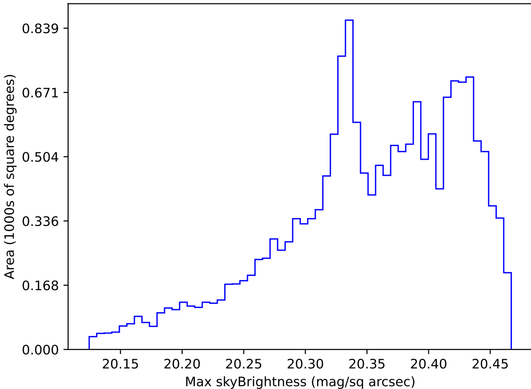
too_ignore_5_1v3.4_10yrs WFD i band: Max skyBrightness
