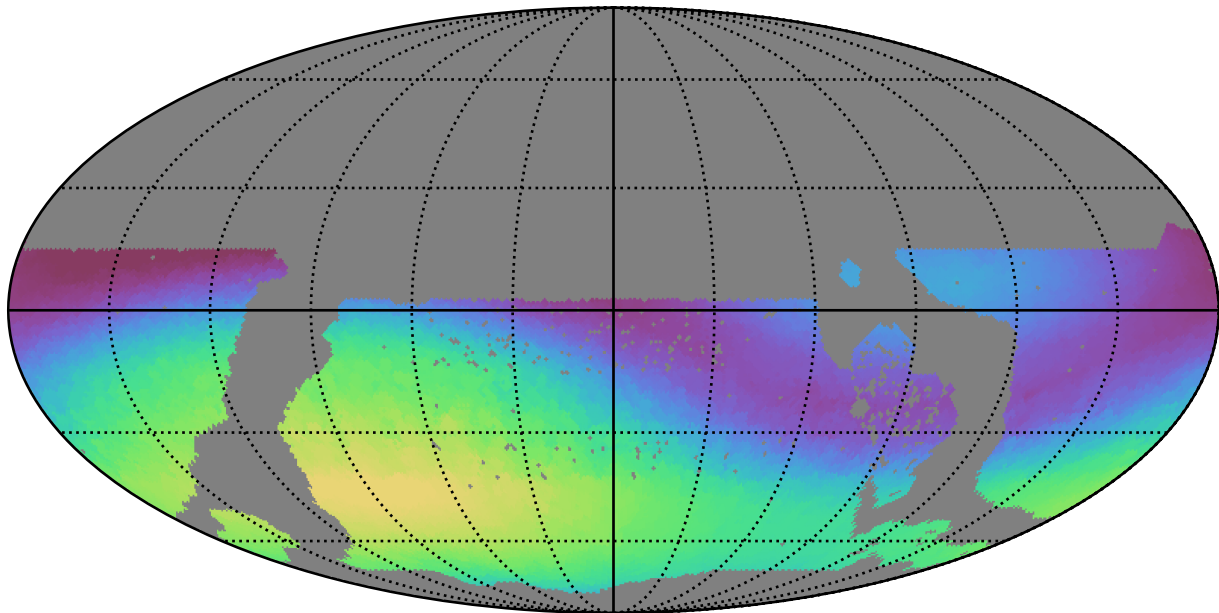
too_ignore_5_1v3.4_10yrs WFD g band: Max skyBrightness
