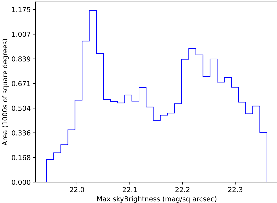
too_ignore_5_1v3.4_10yrs WFD g band: Max skyBrightness
