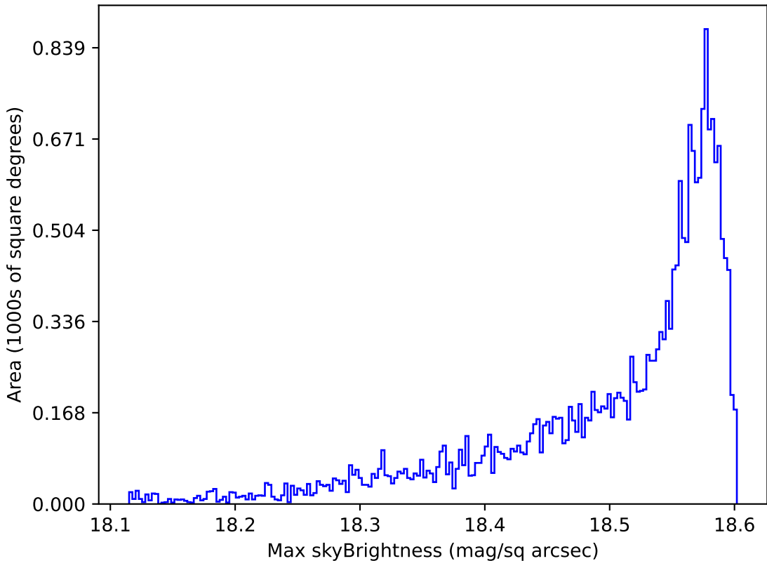
too_ignore_5_1v3.4_10yrs All sky y band: Max skyBrightness
