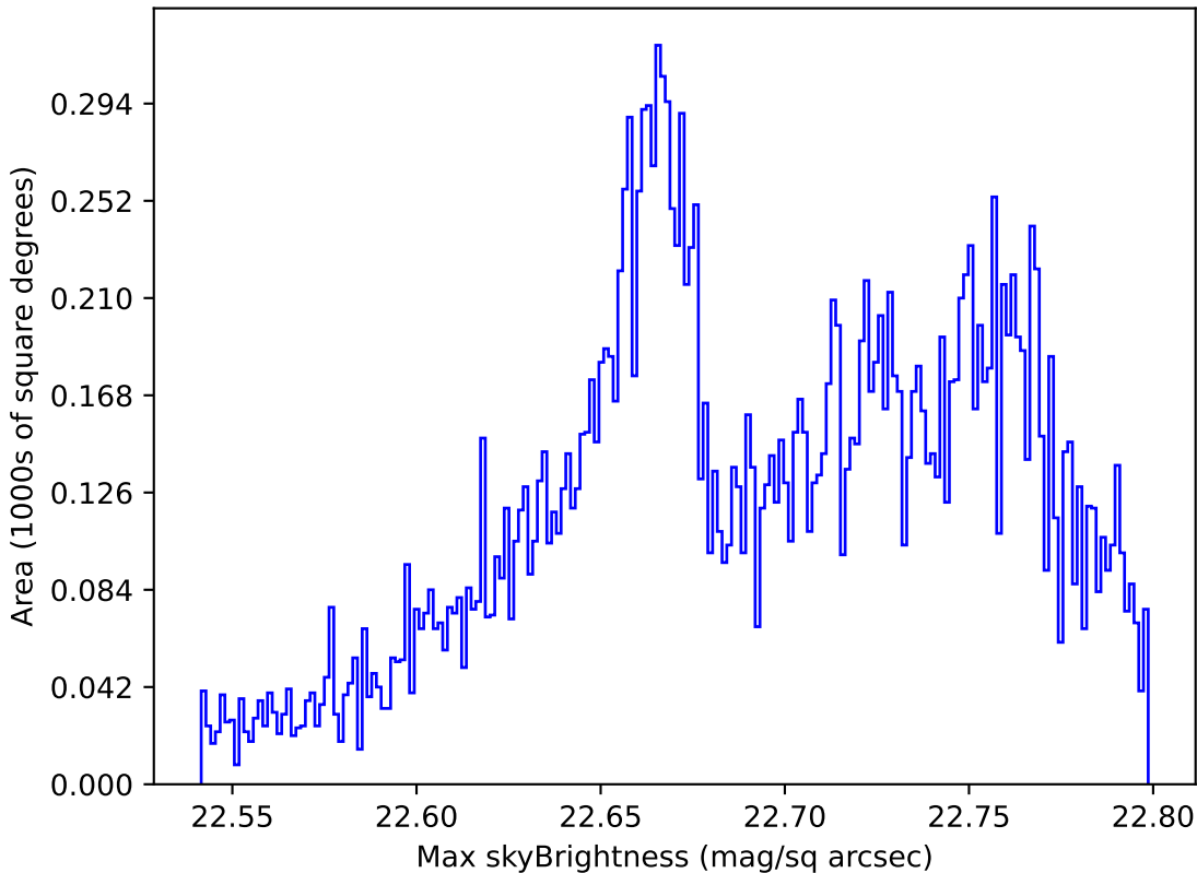
too_ignore_5_1v3.4_10yrs All sky u band: Max skyBrightness
