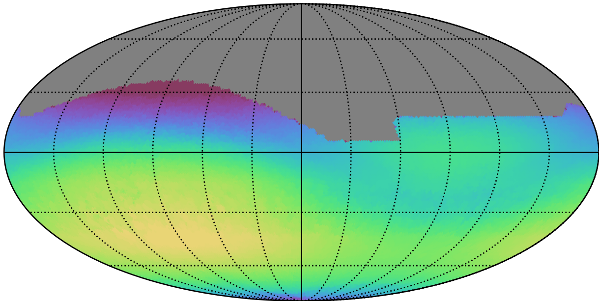
too_ignore_5_1v3.4_10yrs All sky r band: Max skyBrightness
