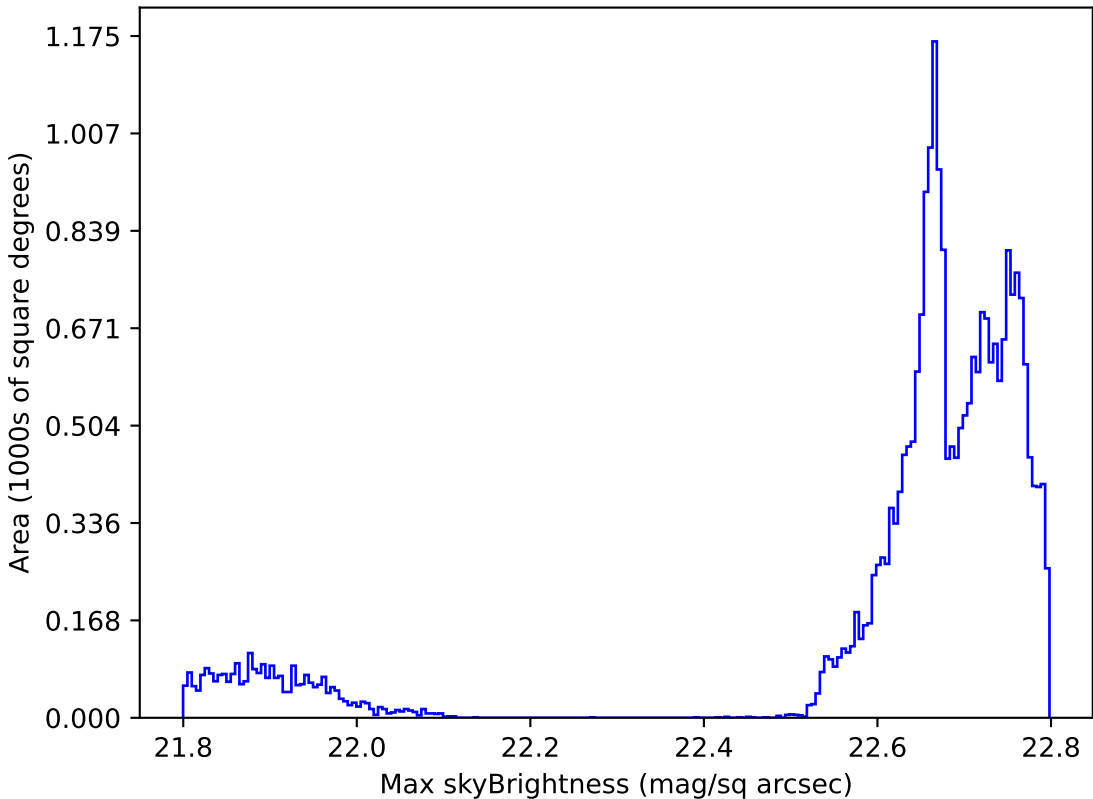
too_ignore_5_1v3.4_10yrs All sky all bands: Max skyBrightness
