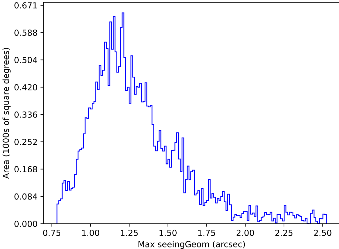
too_ignore_5_1v3.4_10yrs Yr 1 z band: Max seeingGeom
