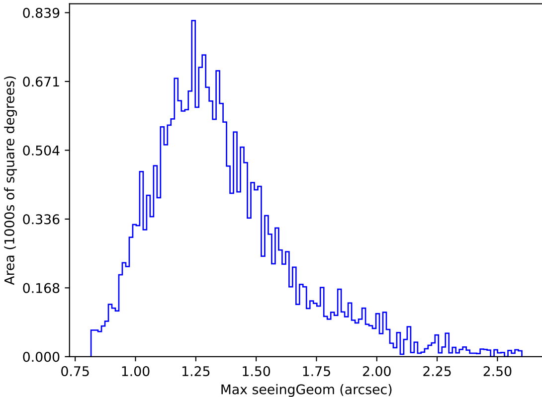
too_ignore_5_1v3.4_10yrs Yr 1 r band: Max seeingGeom
