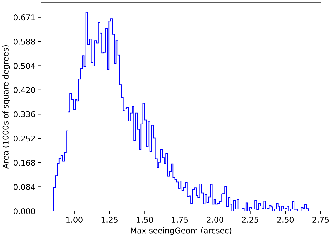
too_ignore_5_1v3.4_10yrs Yr 1 g band: Max seeingGeom
