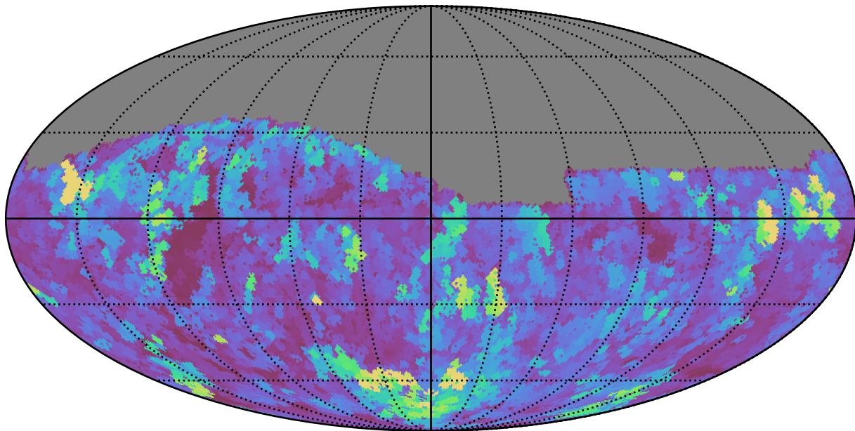
too_ignore_5_1v3.4_10yrs Yr 1 z band: Max seeingEff
