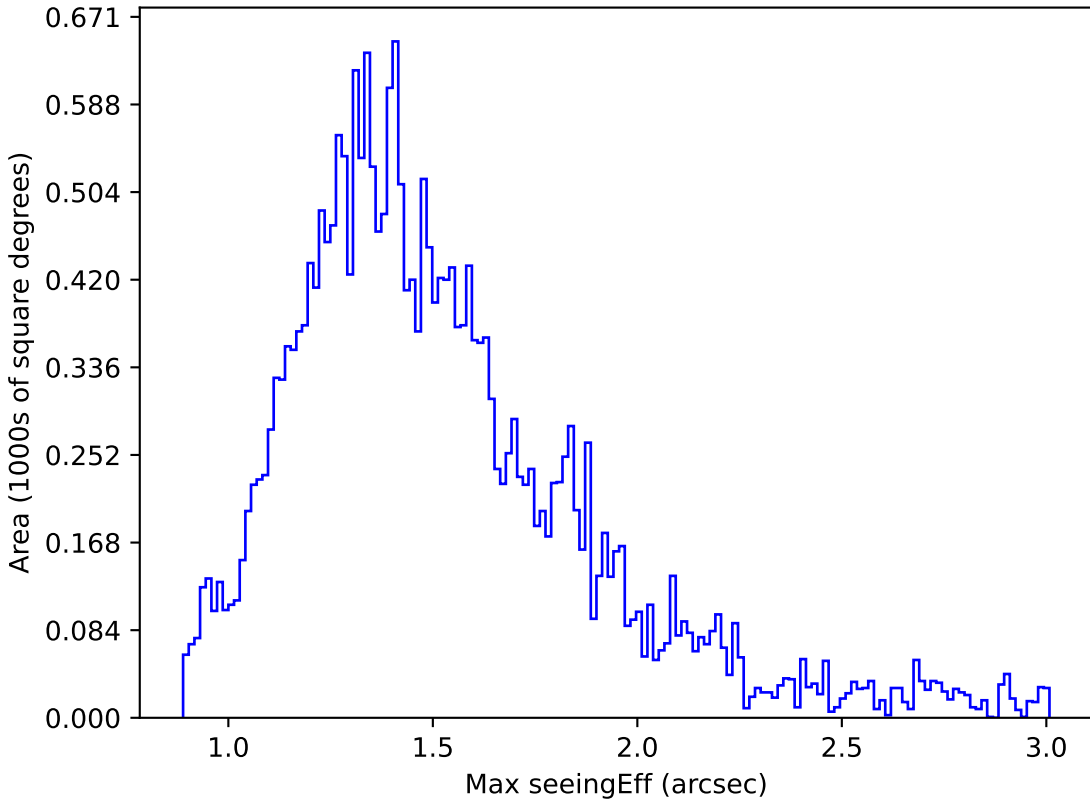
too_ignore_5_1v3.4_10yrs Yr 1 z band: Max seeingEff
