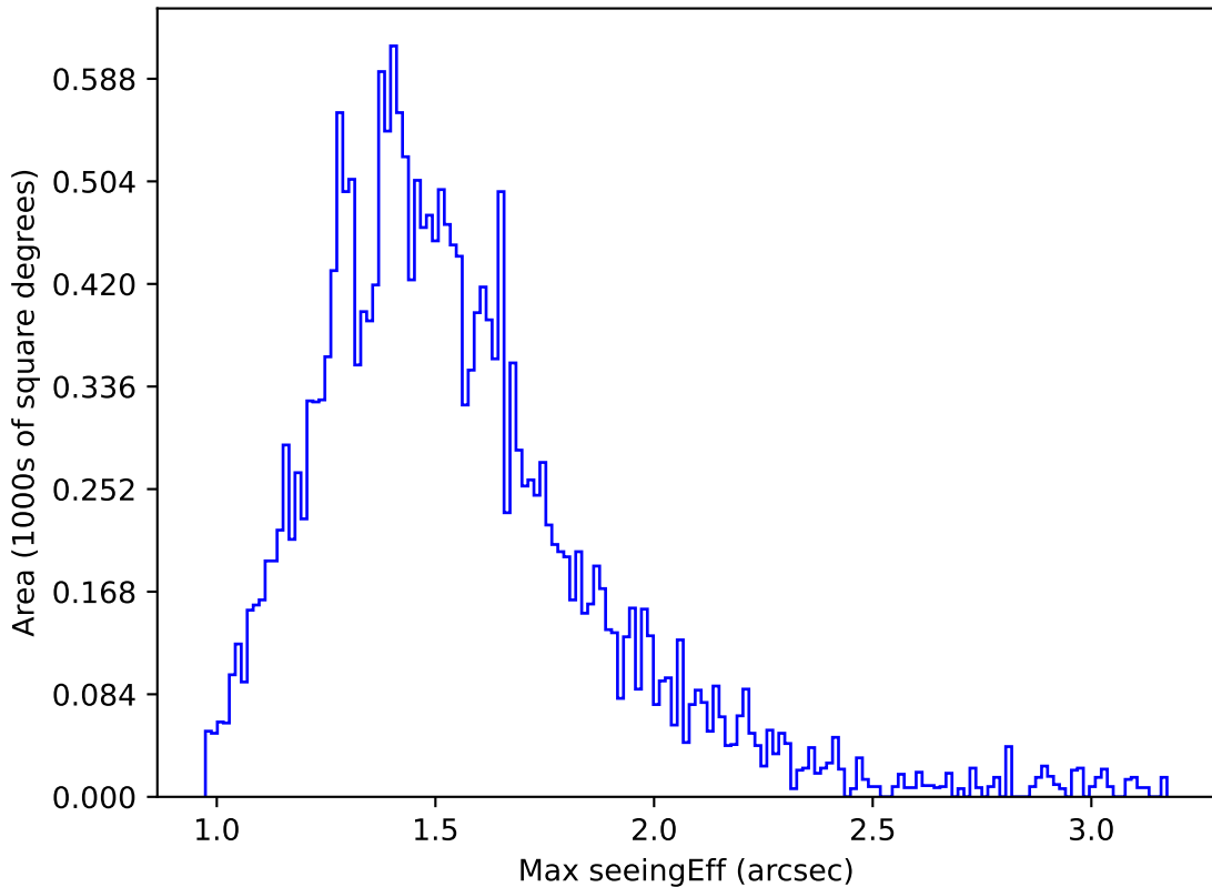
too_ignore_5_1v3.4_10yrs Yr 1 u band: Max seeingEff
