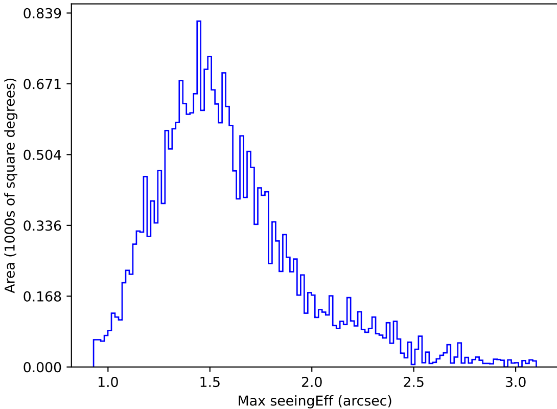
too_ignore_5_1v3.4_10yrs Yr 1 r band: Max seeingEff
